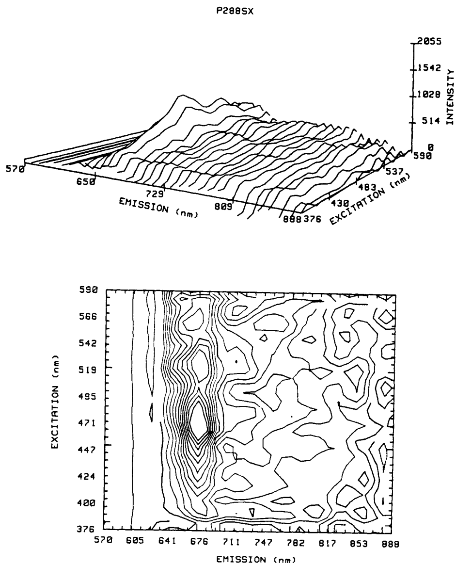
FIG 2 EEM from the Gulf of Mexico.
