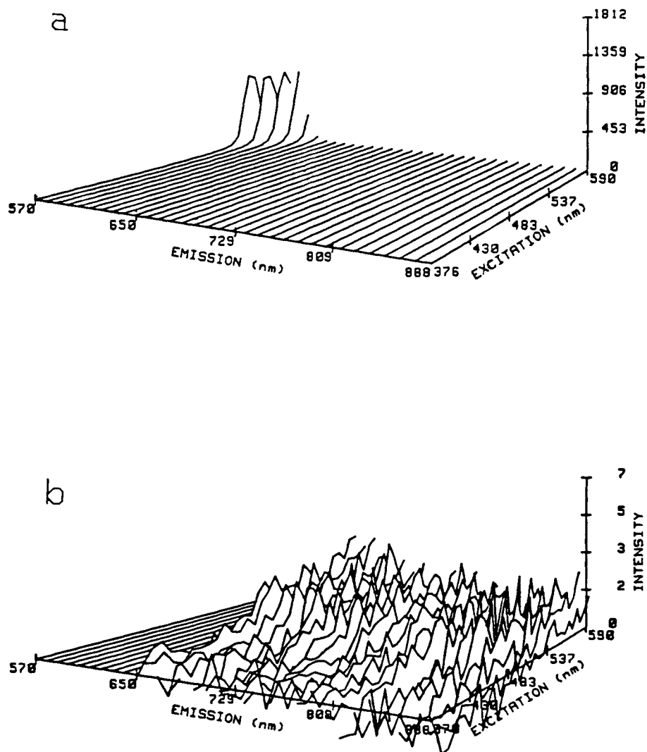
FIG 1 In situ EEM acquired at the Orca Basin in the Gulf of Mexico. a) background subtracted EEM; b) renormalized residual EEM following removal of Rayleigh scattering.
