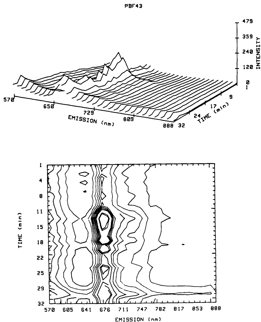
FIG 6 Time-emission matrix (TEM) acquired along the Wilmington and Skidaway Rivers.
